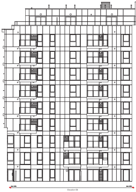
Elevation EB
